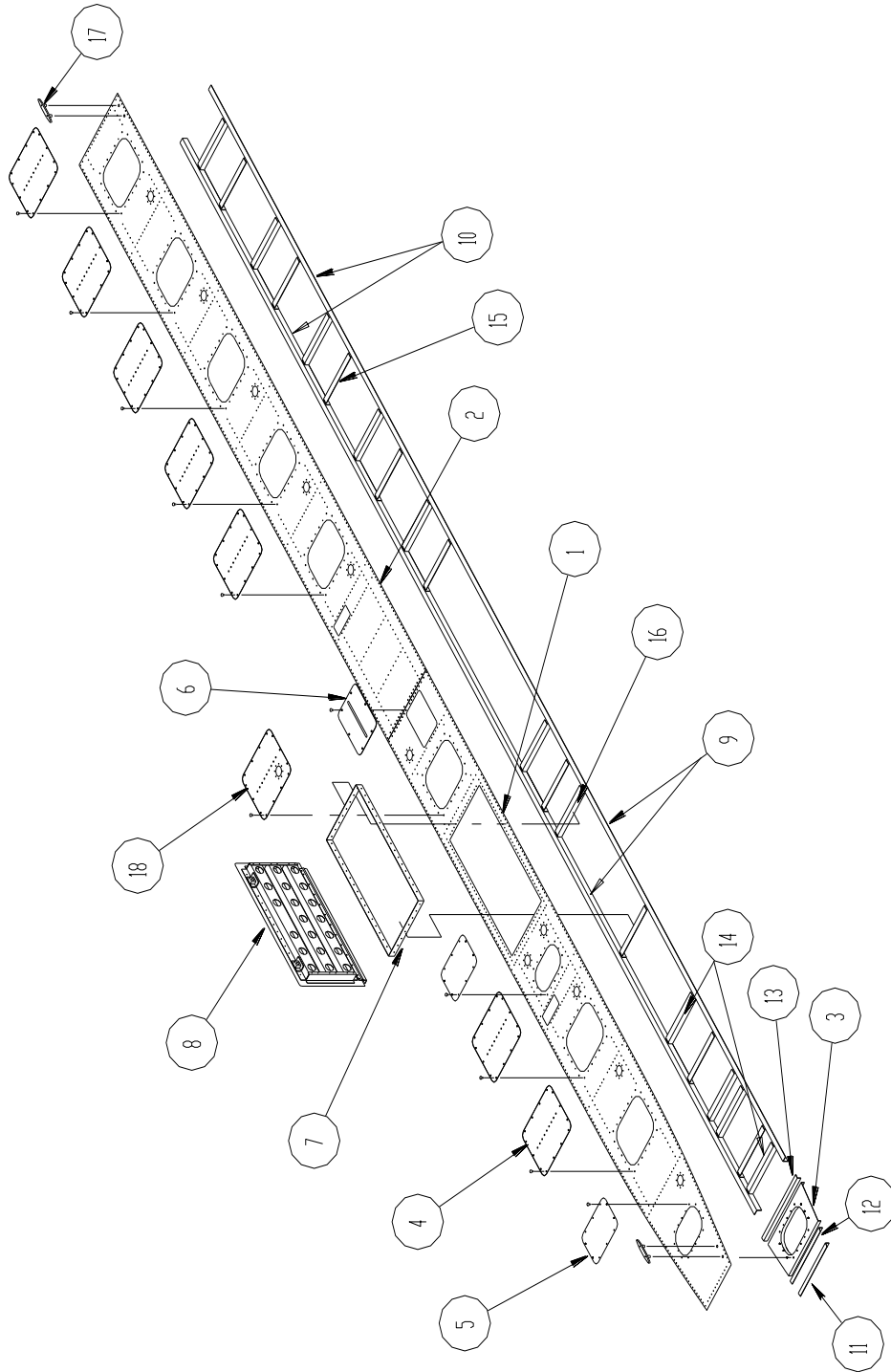
TOP SKIN – HULL – AMPHIBIAN FIGURE 3
