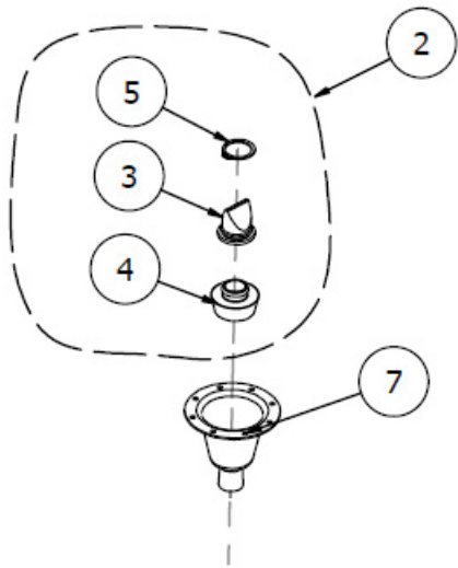
DUCKBILL VALVE RETROFIT
