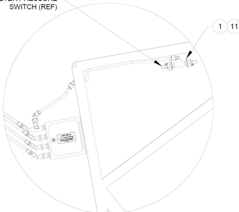
TORQUE PRESSURE SWITCH MVP ENGINE INSTRUMENT SYSTEM
