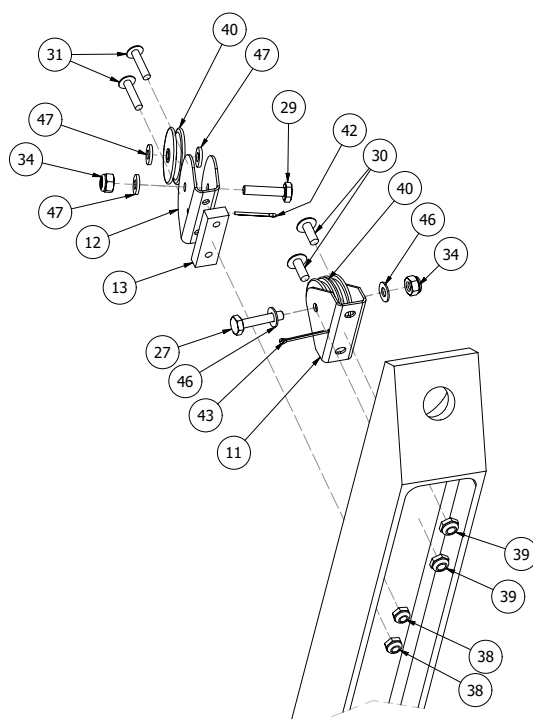
DETAIL A SCALE 1 / 2
