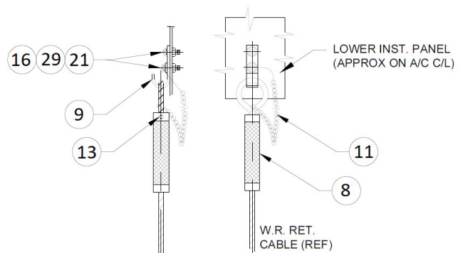
DETAIL E
