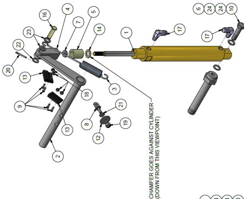
NEW STYLE CLEVIS (SEE SERVICE LETTER 139)
