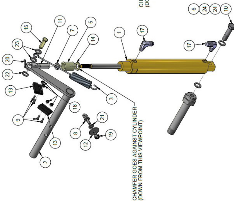
OLD STYLE CLEVIS
