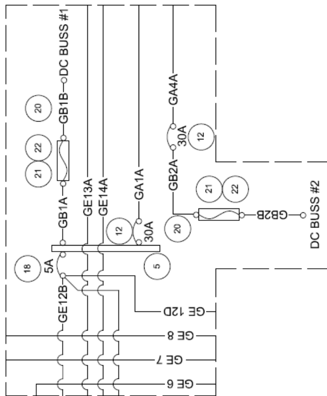
CIRCUIT BREAKER CONFIGURATION "B" ENGINE CONTROL QUADRANT
