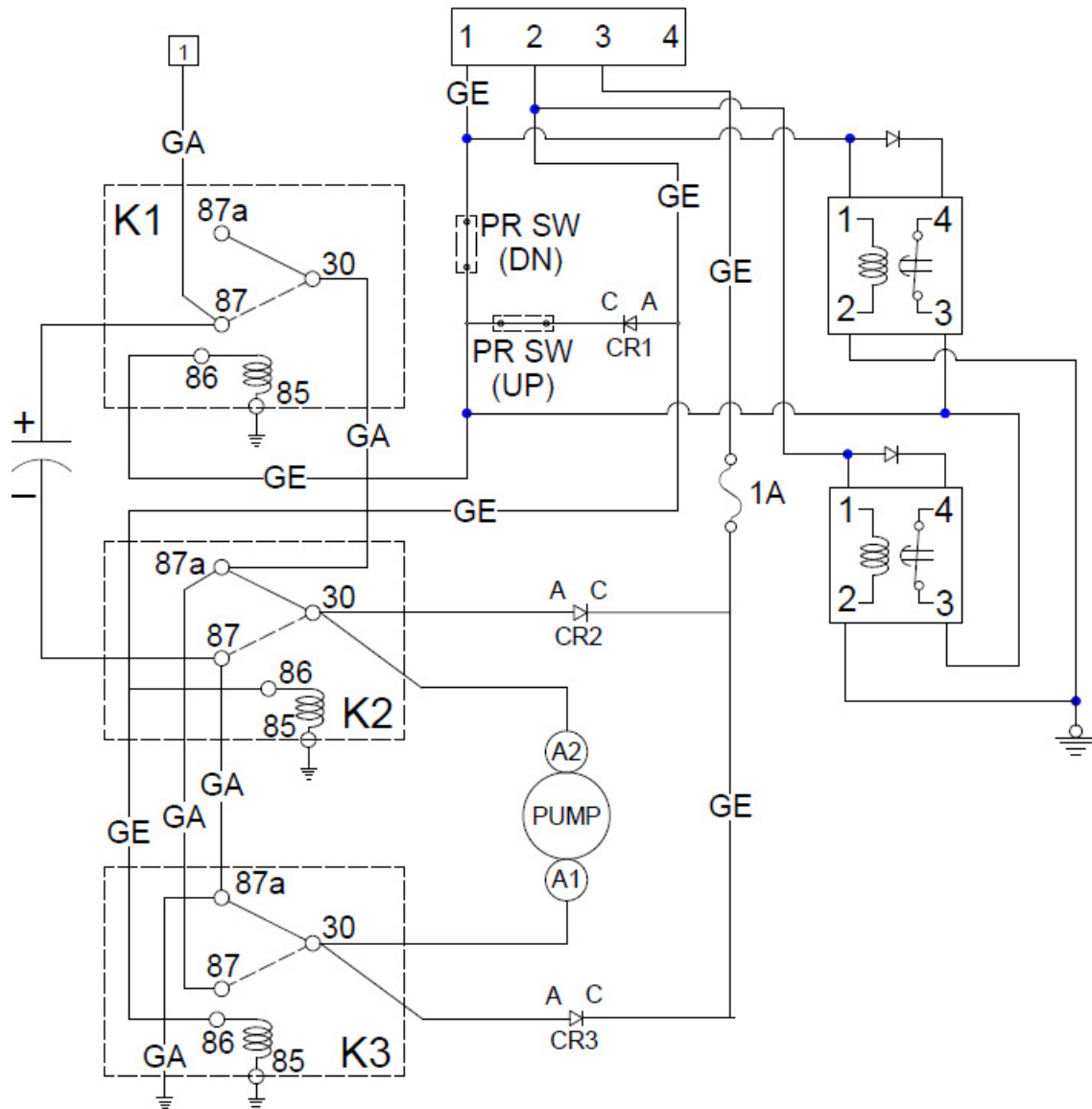
POWER PACK SCHEMATIC (RELAYS SHOWN IN RELAXED CONDITION) 1. GE WIRES 20 GA 2. GA WIRES 12 GA
