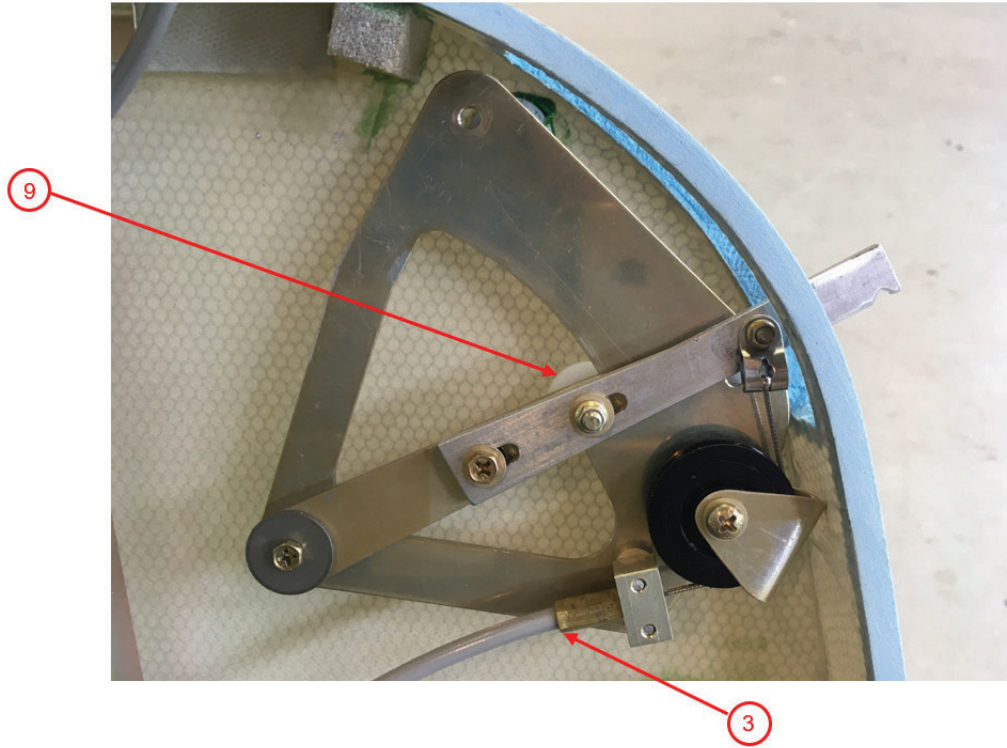
Figure 2 - Lever Brake
