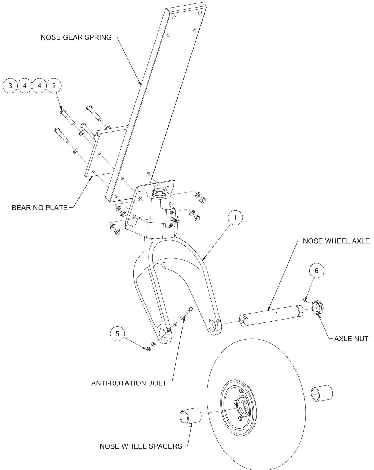
Figure 2 – Install Updated Pivot Block AND Single-Piece Nose Fork
